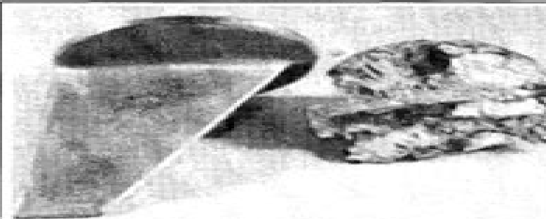
Fig. 22 Such extensive erosion of a trim tab compared with a new tab suggests an electrolysis problem or complete disregard for periodic maintenance
