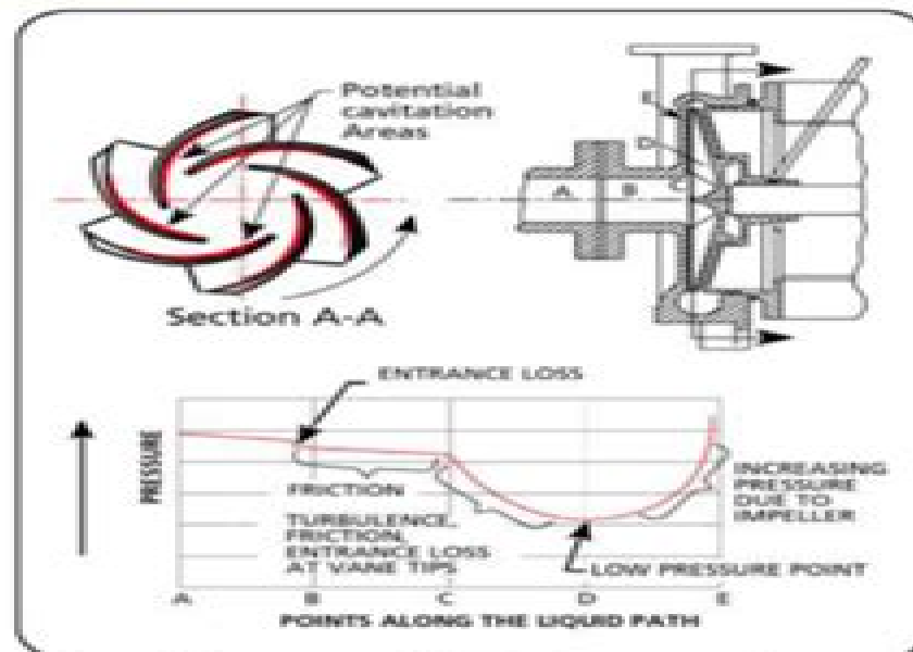
Figure 1 Pressure profile at the pump entrance.
