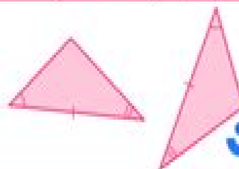
Angle-side-angle (ASA)
