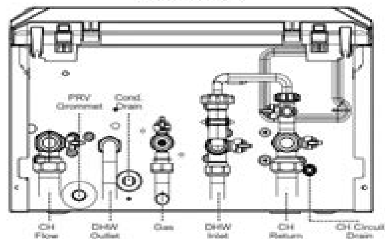
Underside View
