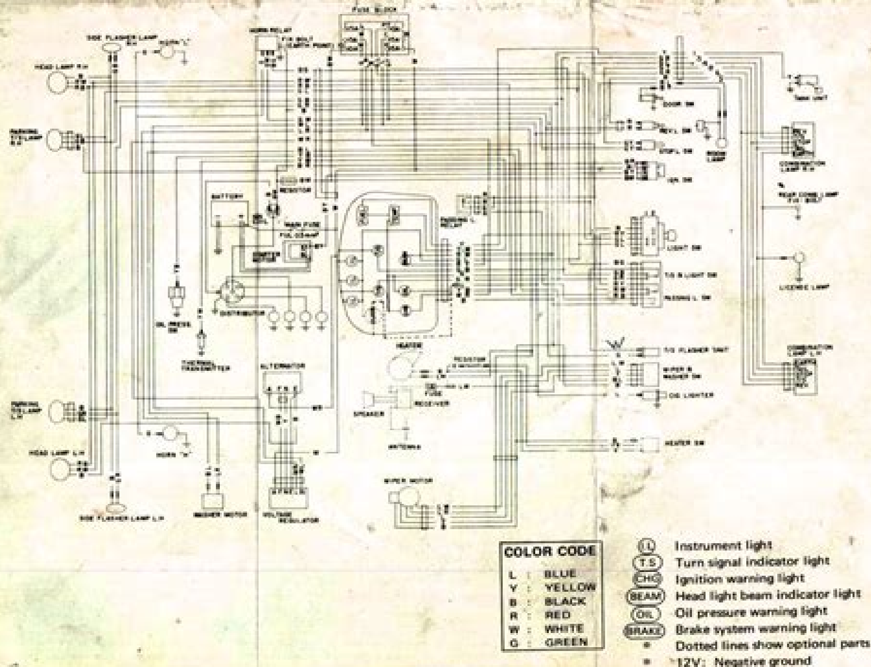
WIRING DIAGRAM DATSUN 1200 (EXCEPT U.S.A. AND CANADA)
