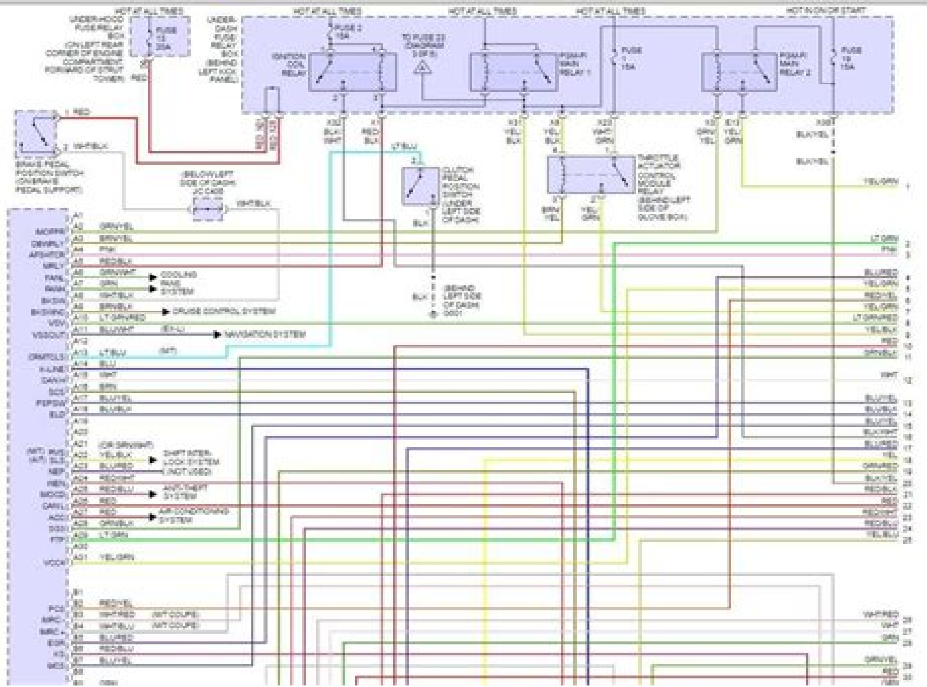
Fig 1: 3.0L Engine Performance Circuit, Except Hybrid (1 of 5)
