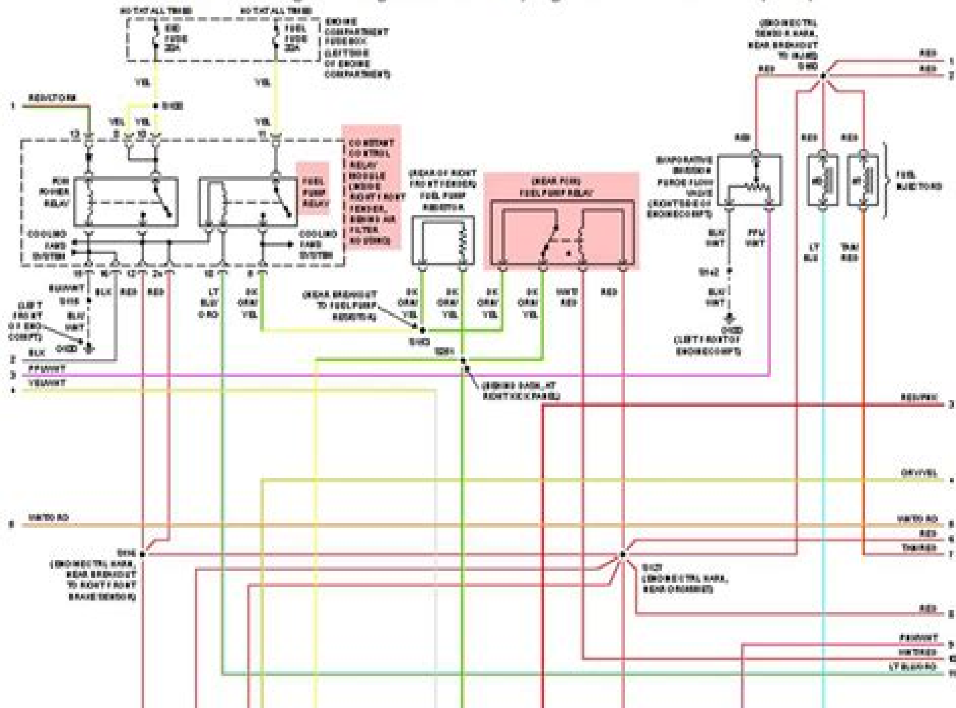
1998 Ford Mustang Cobra-Fig. 17: 4.6L DOHC, Engine Performance Circuits (2 of 3)
