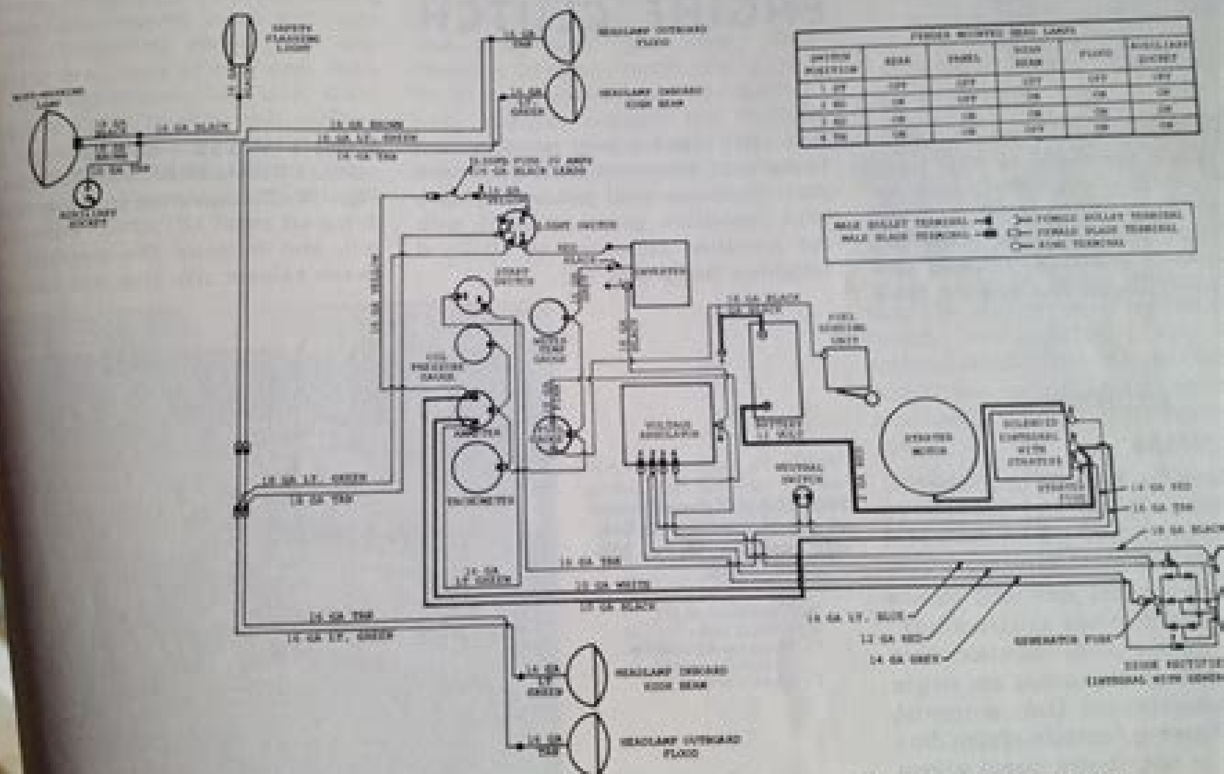
Fig. 194—Wiring diagram for MF135 diesel equipped with alternator. Other late models are similar.
