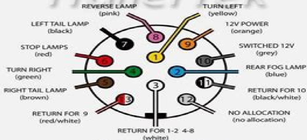
13pin Socket Wiring
