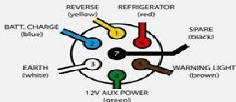
7pin Socket Wiring 12S (Suplimentary)
