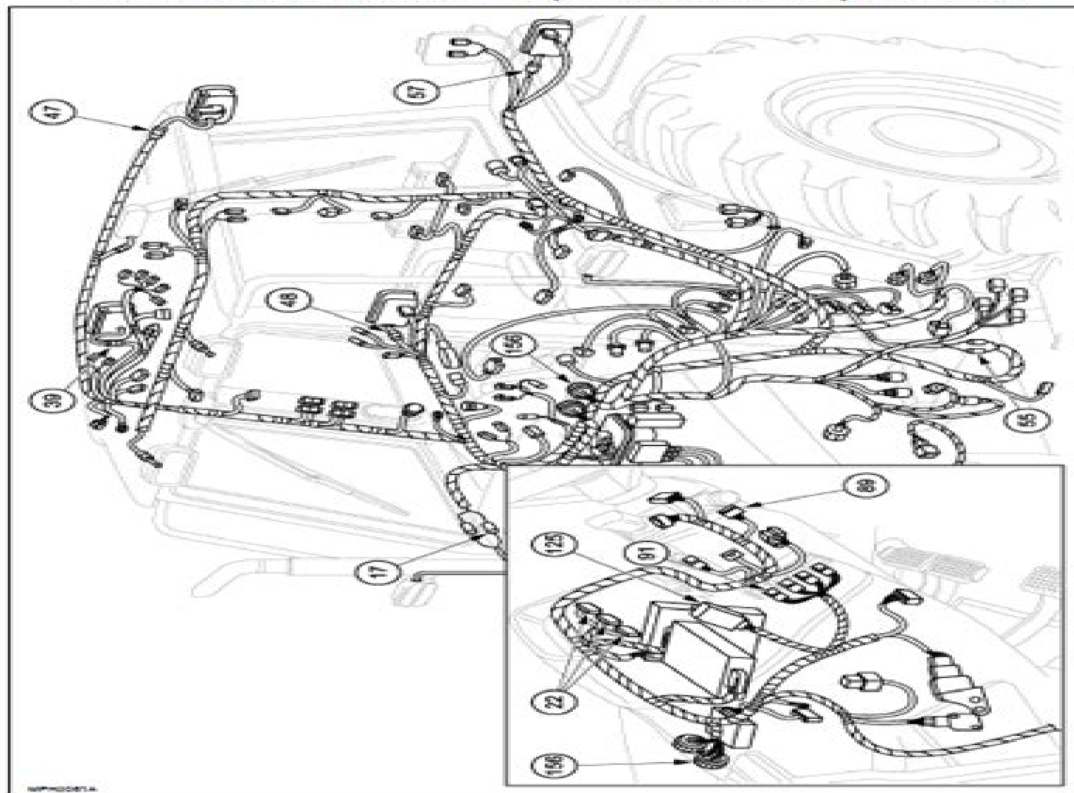
WIRING DIAGRAM C - DUAL COMMAND (2 SPEED POWER SHIFT) CAB VERSION
