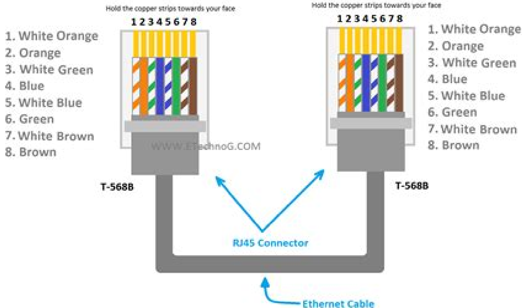
Ethernet Cable Wiring Diagram(T-568B)
