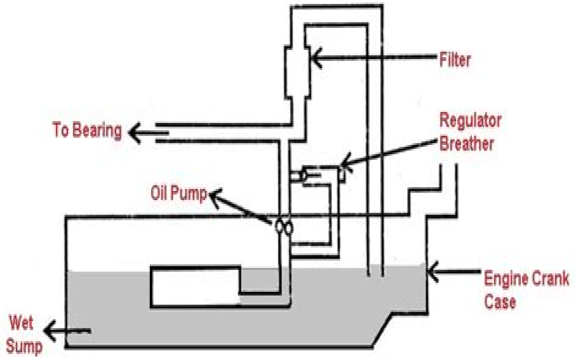
Wet Sump Lubrication System
