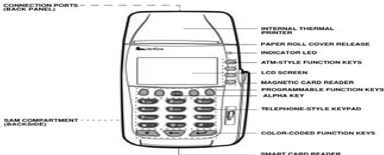
Figure 2 Omni 37xx Terminal Features (Front Panel)
