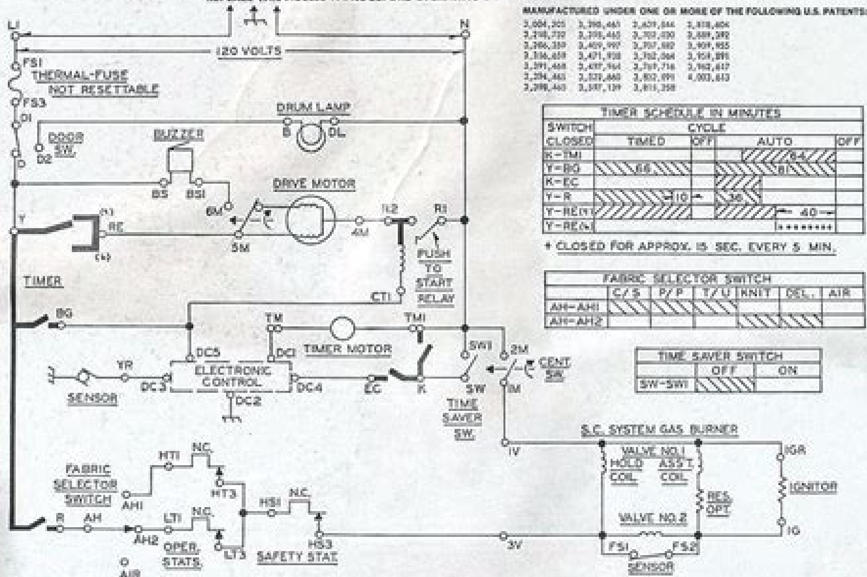
GAS DRYER WIRING DIAGRAM
