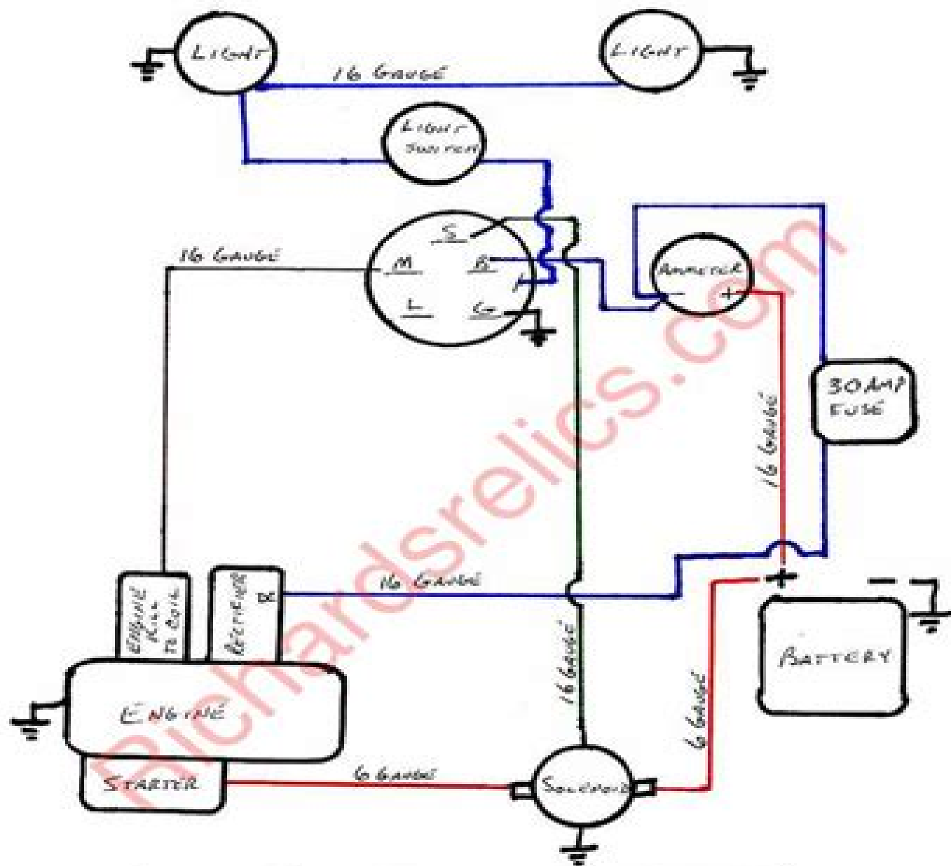
HUSTLER BRIGGS & STRATTON 18HP WIRING IGNITION SWITCH 3 POSITION #399
