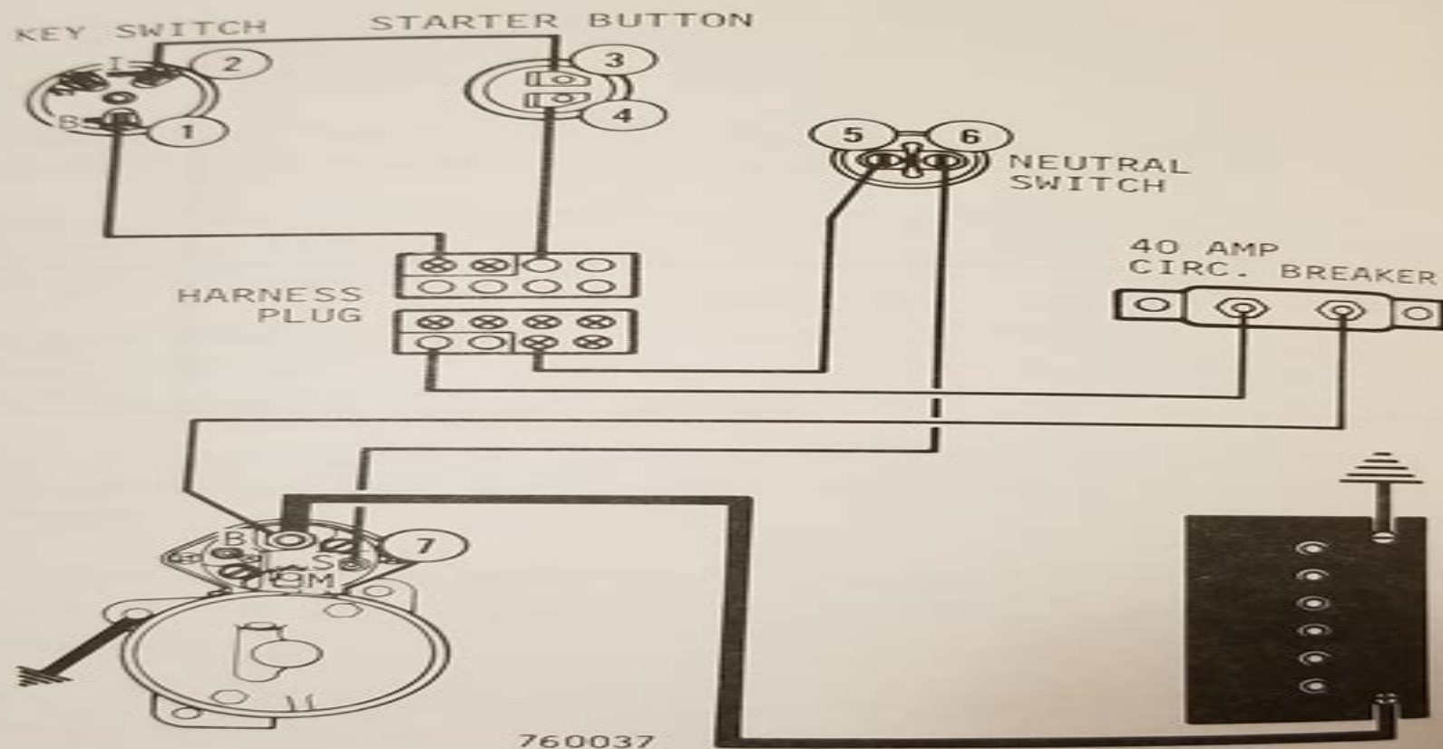
Figure 2 - Starter Circuit
