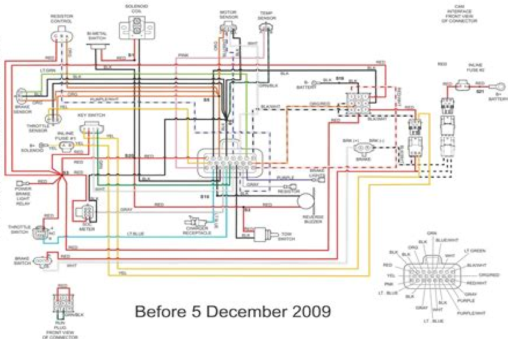
Fig. 31 Main Wiring Diagram (before 5 December 2009)
