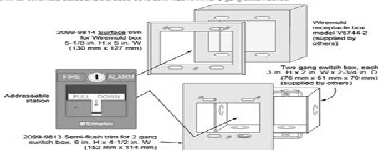
Figure 4: Addressable manual station, additional mounting information
