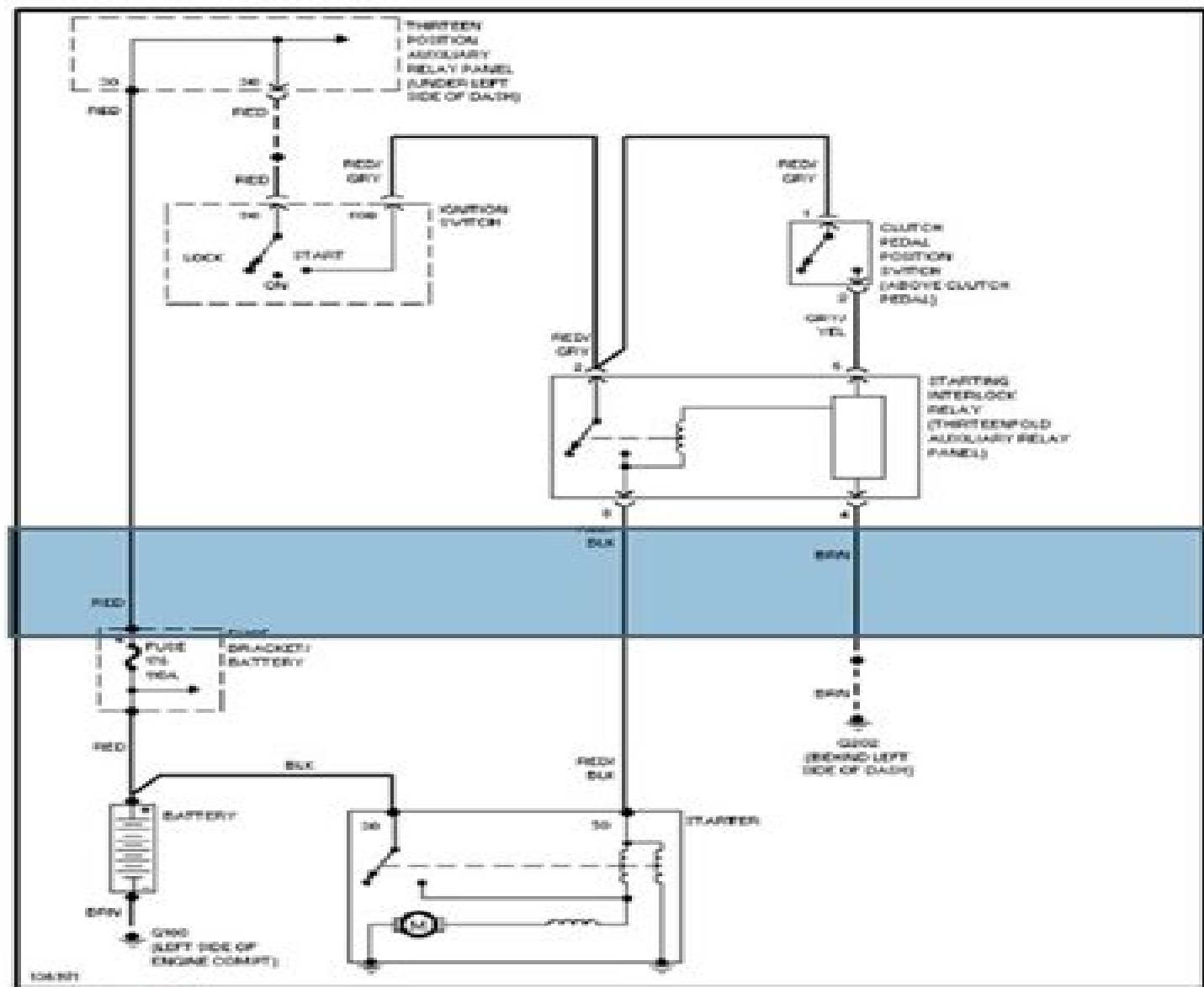
Starting Circuit, M/T
