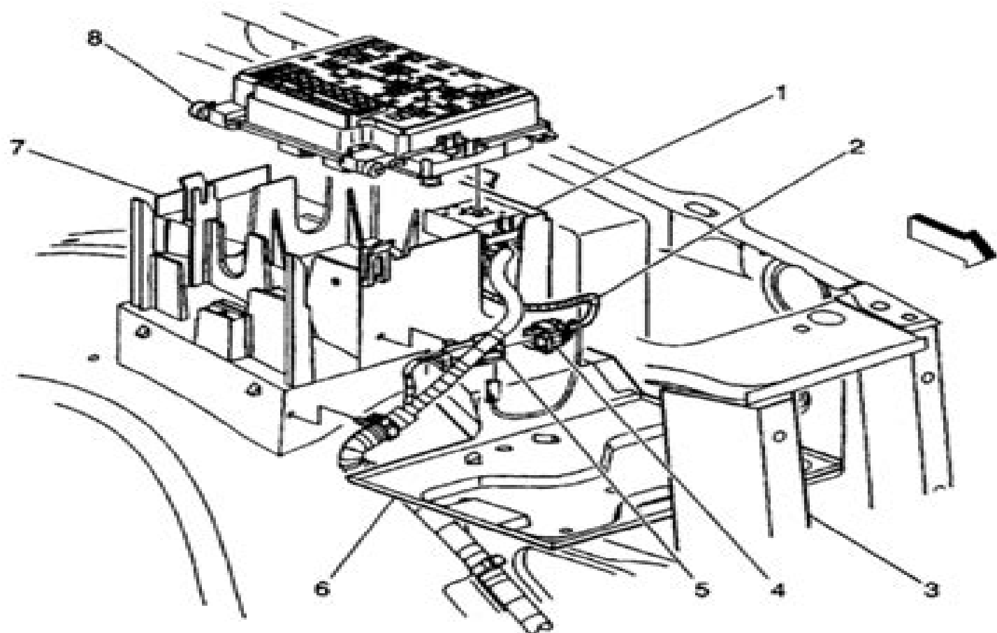
Fig 7: Locating Engine Wiring Harness Junction Block
