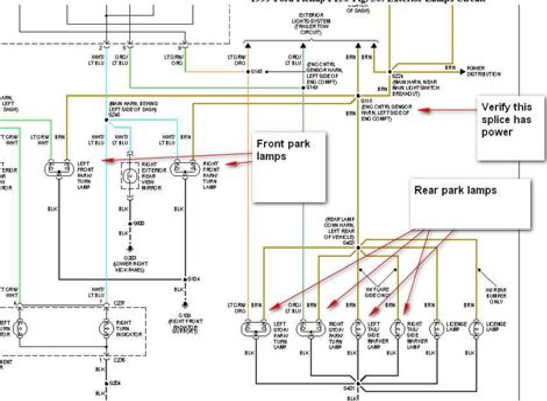
1999 Ford Pickup F150-Fig. 30: Exterior Lamps Circuit
