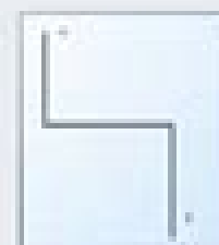
Binary Association
