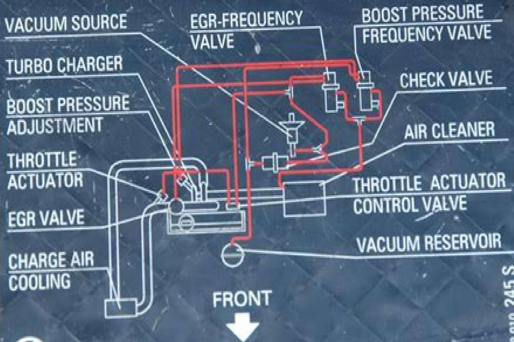
VACUUM HOSE ROUTING DIAGRAM
