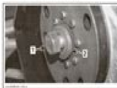
FIGURE 2 1 Drive pulley retaining screw 2 Conical spring washer
