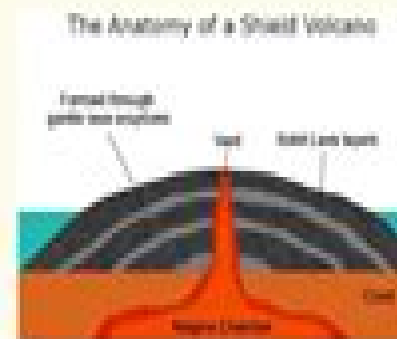
Shield Volcano Diagram
