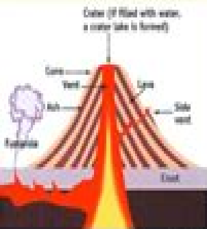
Composite Volcano Diagram
