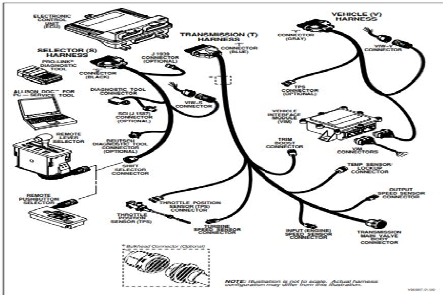
Figure 1-2. CEC2 Components
