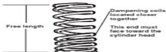
Fig. T910—Valve spring must be installed with dampening coil end positioned against the cylinder head.
