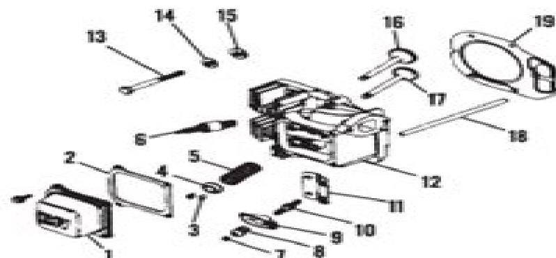
Fig. T907—Exploded view of cylinder head assembly.
