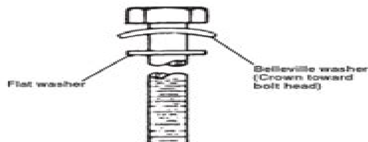
Fig. T908—Install Belleville washer on head bolt with crown toward bolt head. Install flat washer with sharp edge toward bolt head.
