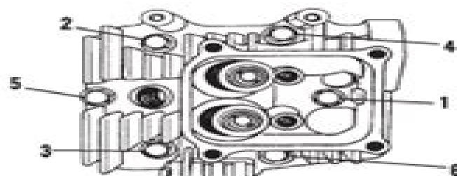
Fig. T909—Tighten cylinder head bolts in sequence shown.
