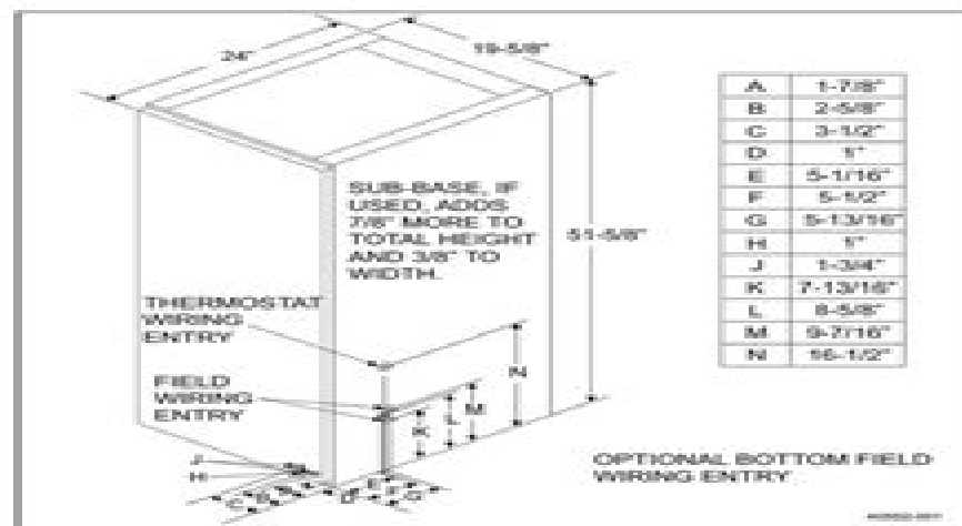
FIGURE 1: Furnace Dimensions
