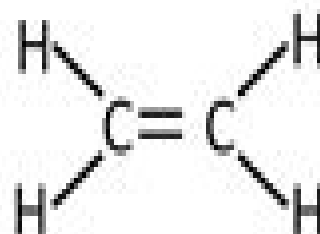
Ethene
