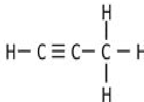
Propyne
