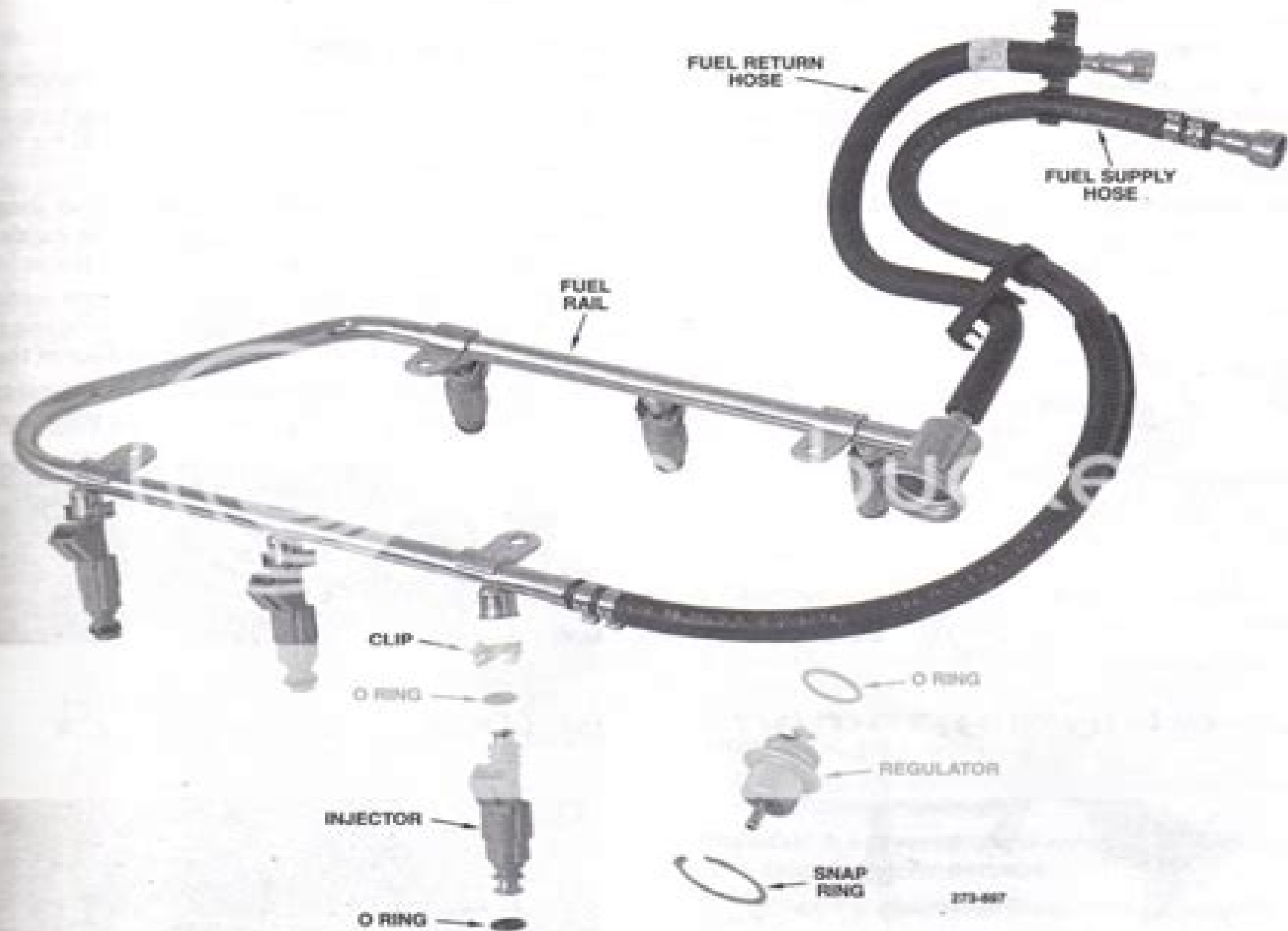
Fuel rail and associated components. Standard models.
