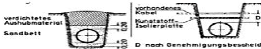
FIGURE 2.2-5: Crossing profiles and line alignments
