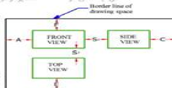
Fig. 6.21 Laying out a three view drawing
