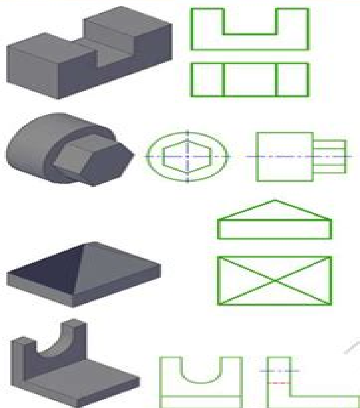
Fig. 6.19 Examples of two view drawings
