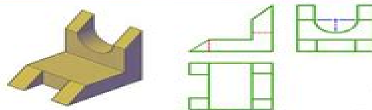
Fig. 6.20 An example of a three-view drawing
