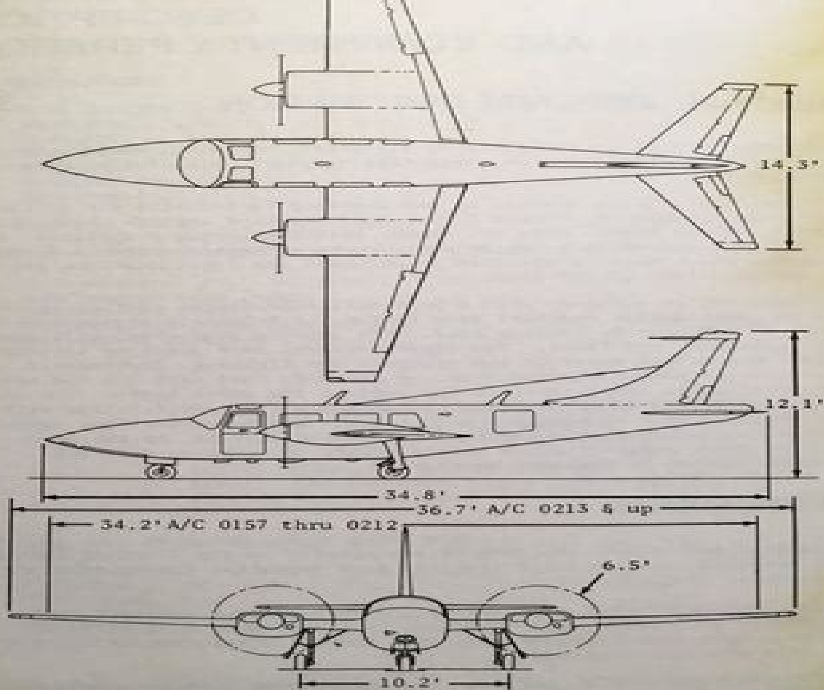
Figure 1-1. General Dimensions
