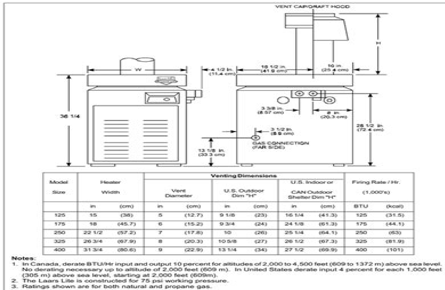
Figure 1. General Configuration.
