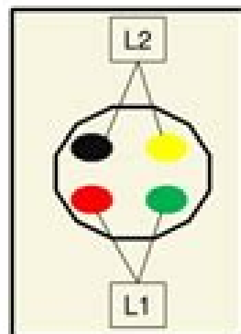
Back-side of Telephone wall plate
