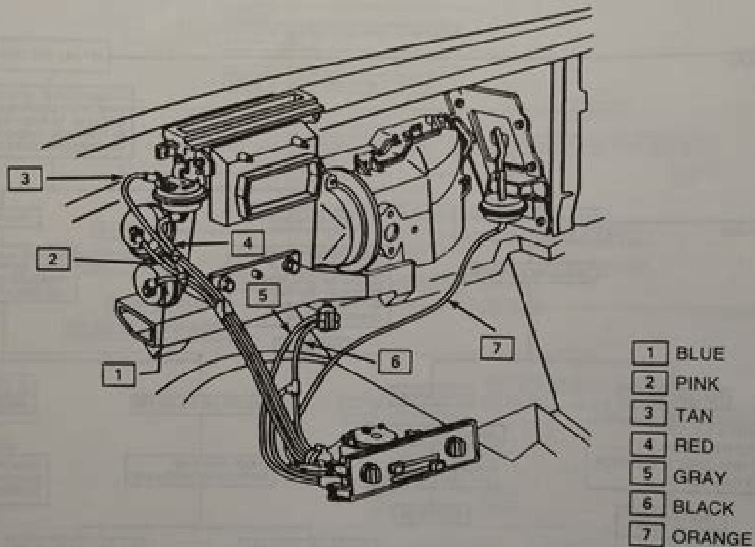
Fig. 1B-12--C60 Interior Vacuum Line Routing
