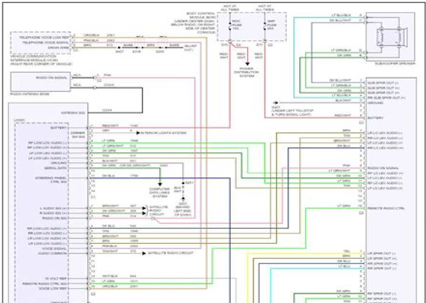
Fig 1: Radio Circuit, W/ Amplifier
