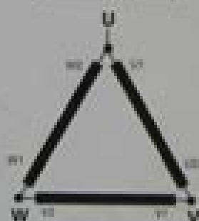
Delta 3Ph 4W Output Terminals (U, V, W)
