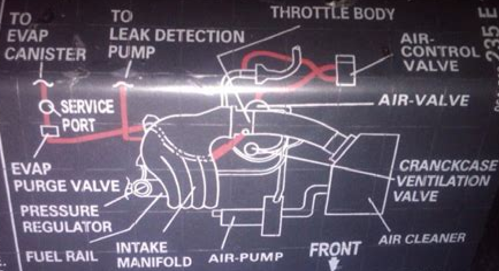
VACUUM HOSE ROUTING DIAGRAM
