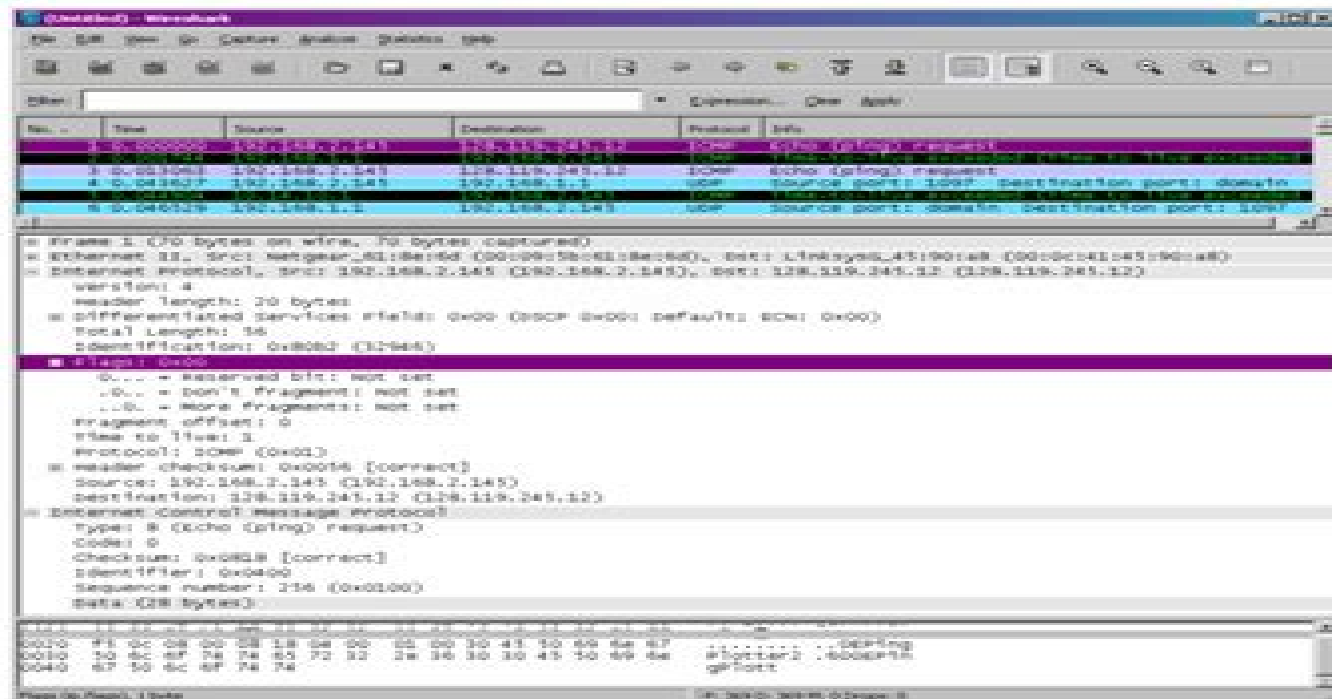
Fig. 1 ICMP Echo Request message IP information
