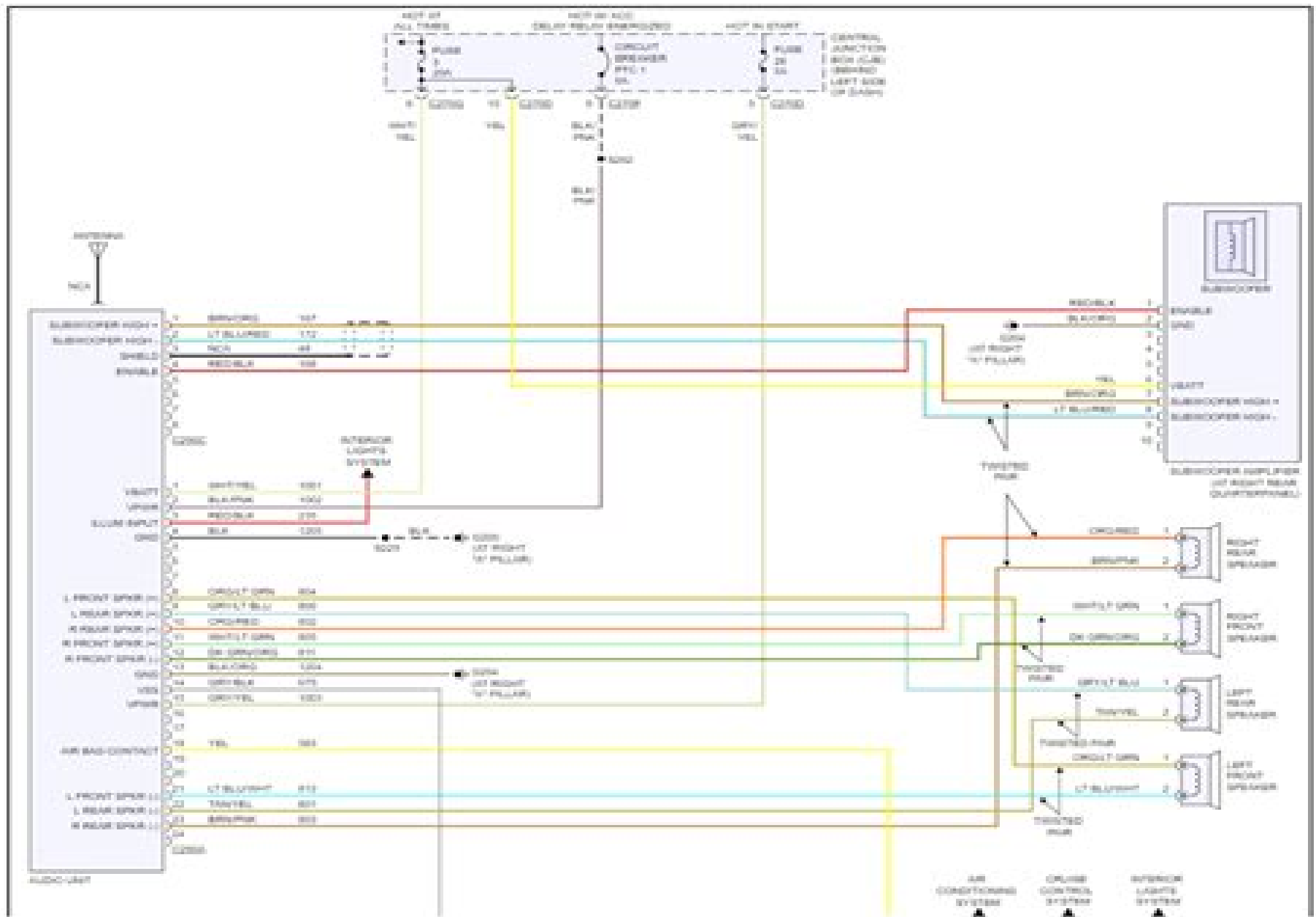
Fig 1: Radio Circuit, W/ Audiophile System
