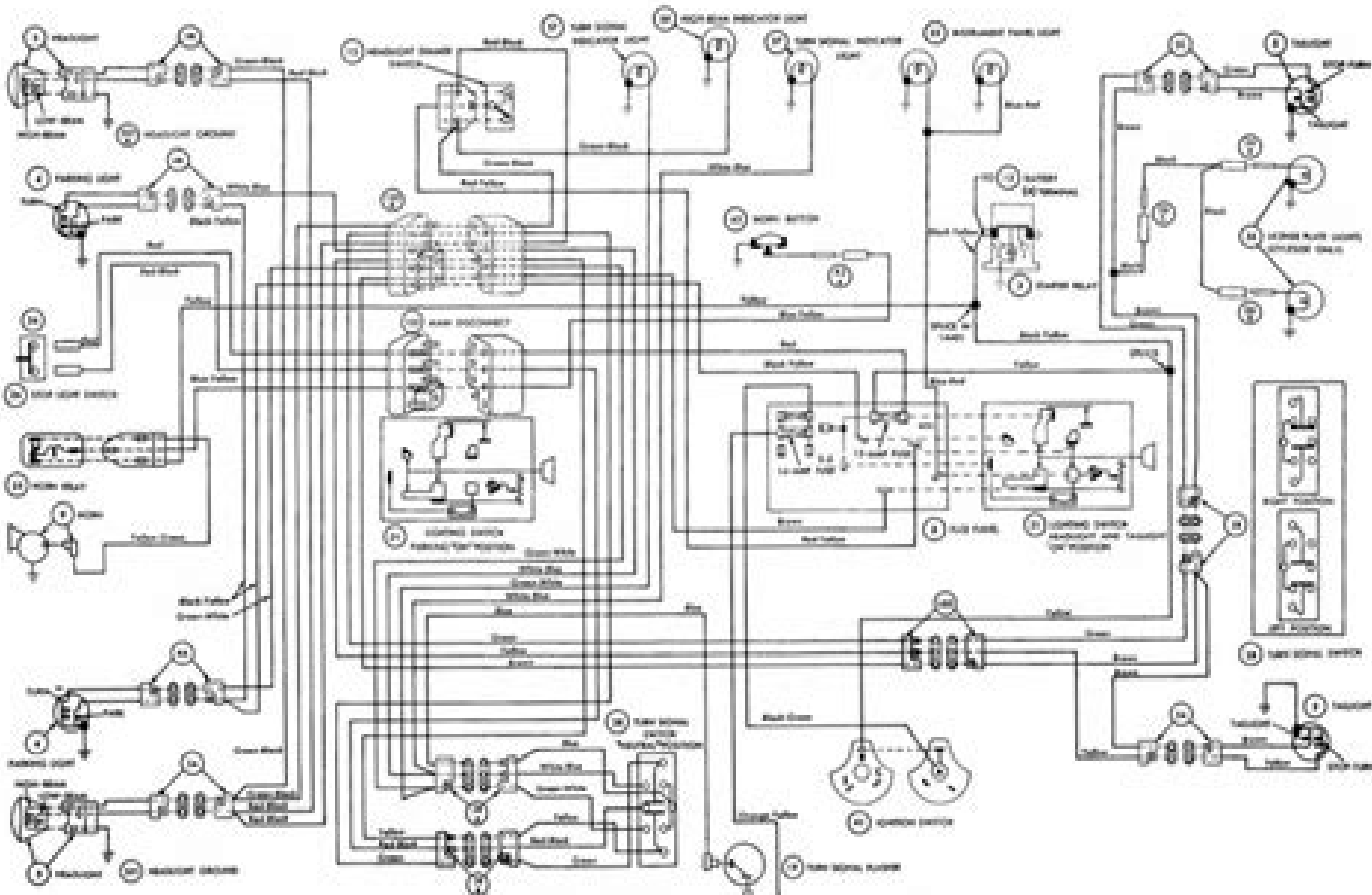
1964 F-100 THRU F-750 SERIES TRUCKS EXTERIOR LIGHTING, TURN SIGNALS AND HORN SCHEMATIC
