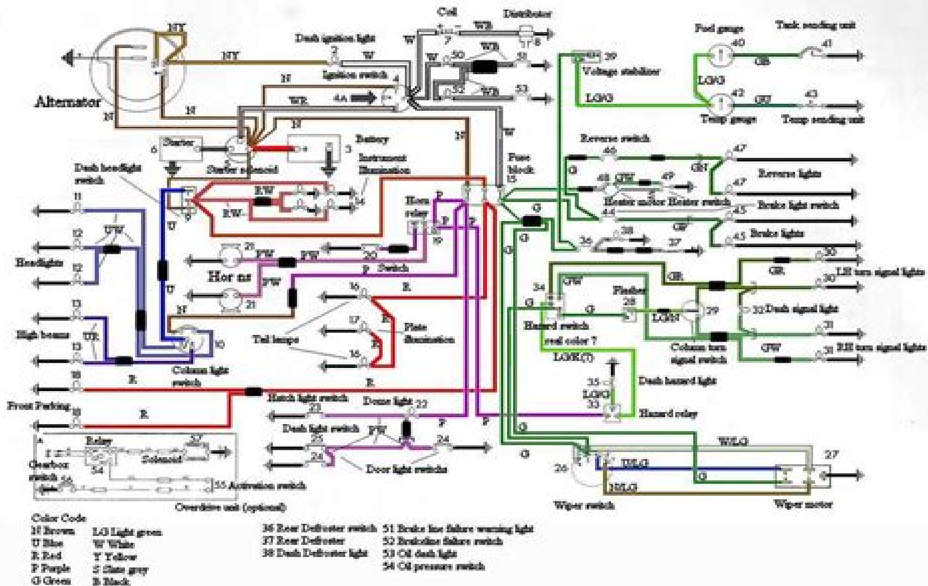
Triumph GT6+ Wiring Diagram
