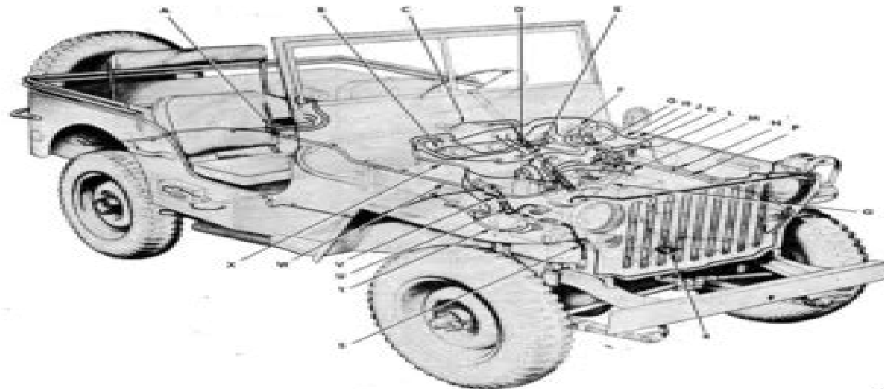
FIGURE 06-12—WIRING INSTALLATION
