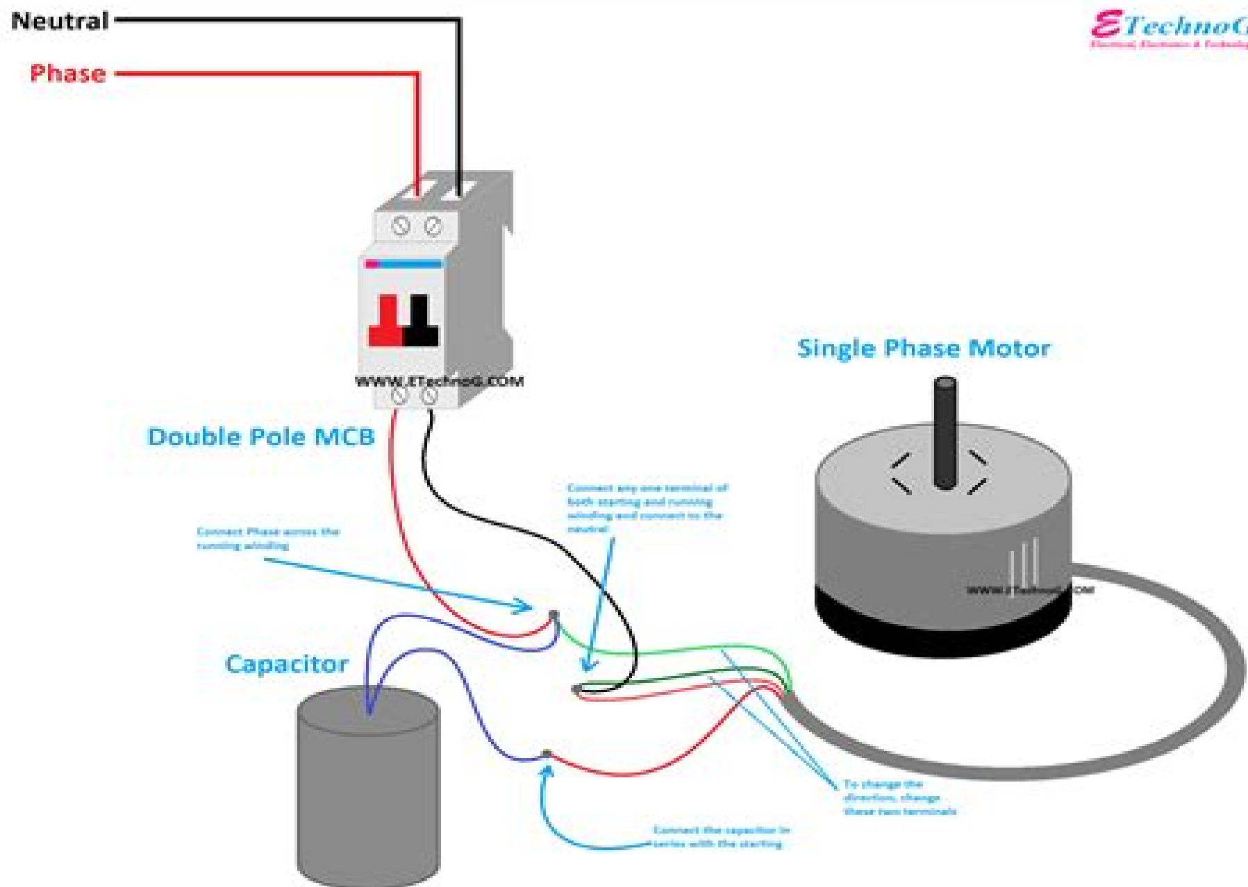
Single Phase Motor Connection Diagram and Wiring Procedure
