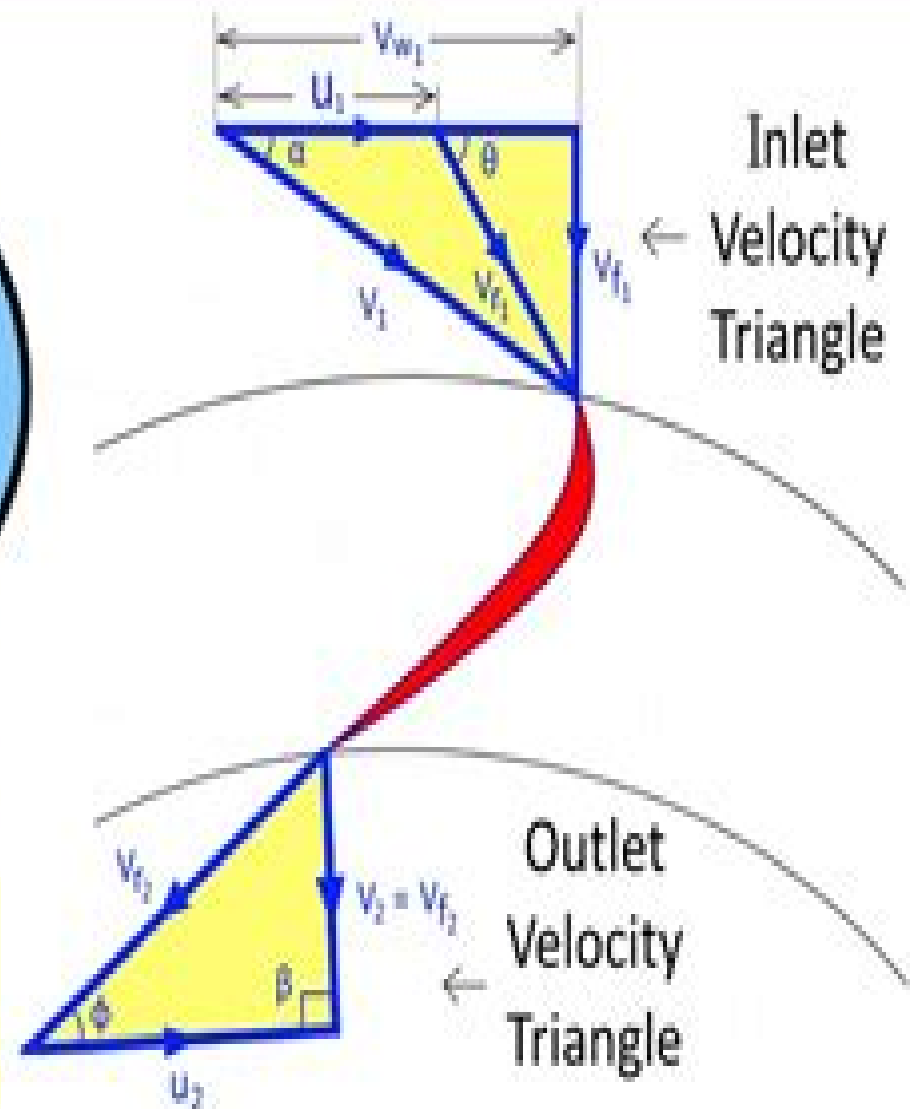
Francis Turbine
