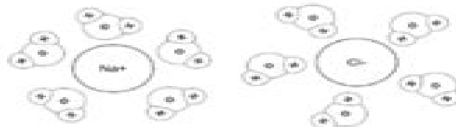
Figure 3: Hydration Spheres
