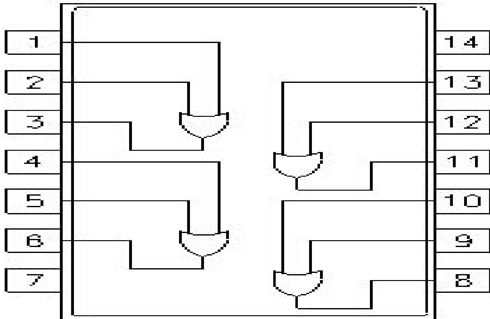
7432 Quad 2-Input OR Gate
