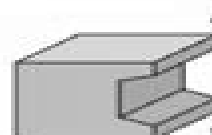
Nonregular, Concave Polyhedron
