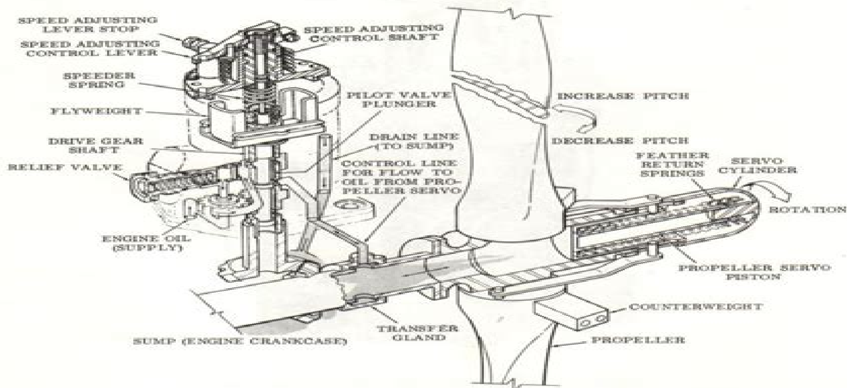
Figure 2. Schematic Diagram of Operation (Pressure to Decrease Pitch Only)
